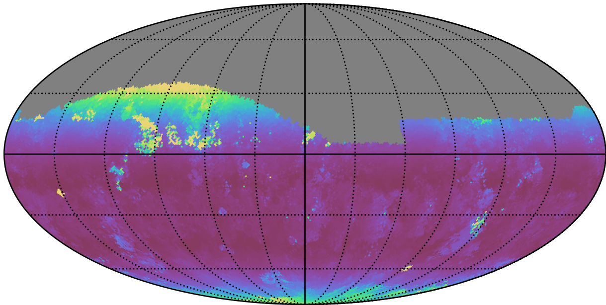
too_elab_r16_d2_griz_v3.4_10yrs Yr 1 z band: Median airmass
