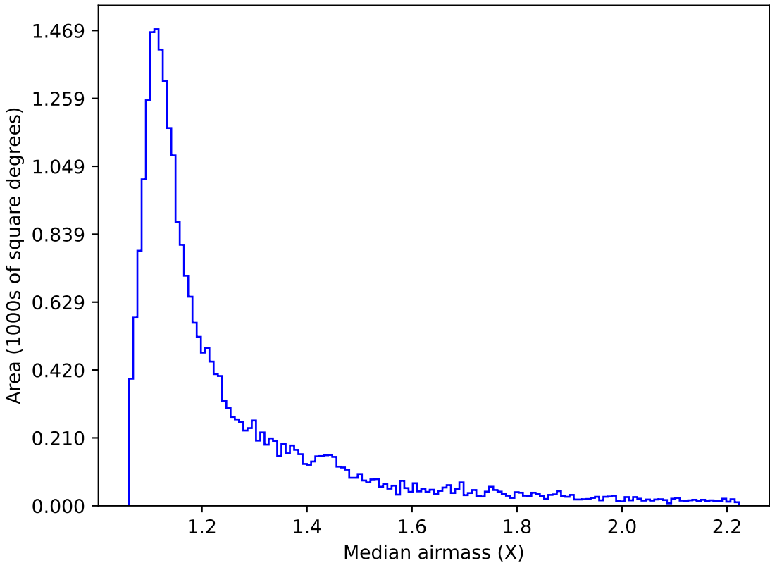
too_elab_r16_d2_griz_v3.4_10yrs Yr 1 z band: Median airmass
