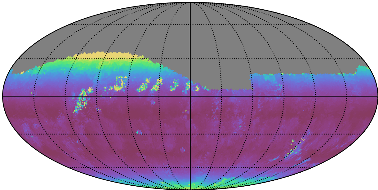
too_elab_r16_d2_griz_v3.4_10yrs Yr 1 r band: Median airmass
