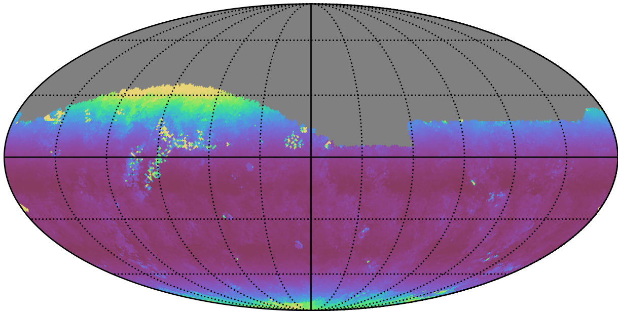
too_elab_r16_d2_griz_v3.4_10yrs Yr 1 i band: Median airmass
