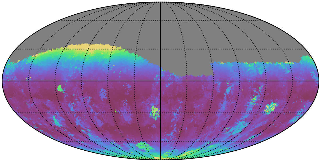
too_elab_r16_d2_griz_v3.4_10yrs Yr 1 g band: Median airmass
