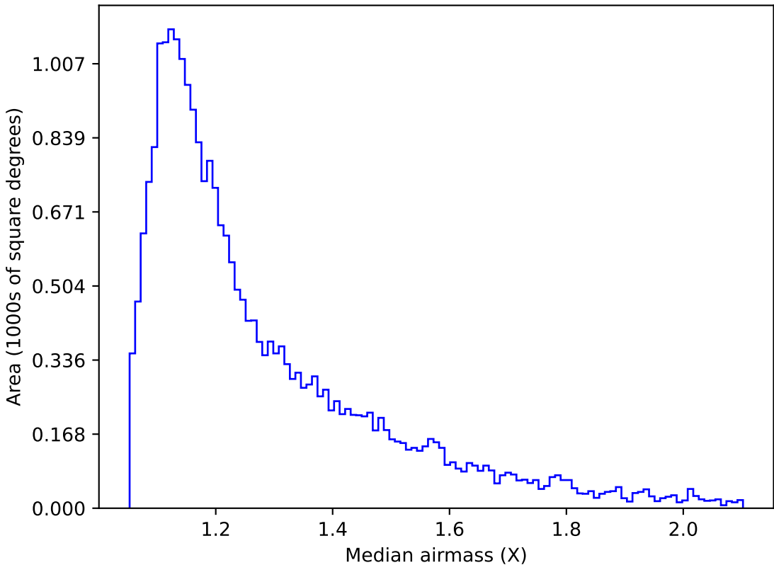
too_elab_r16_d2_griz_v3.4_10yrs Yr 1 g band: Median airmass
