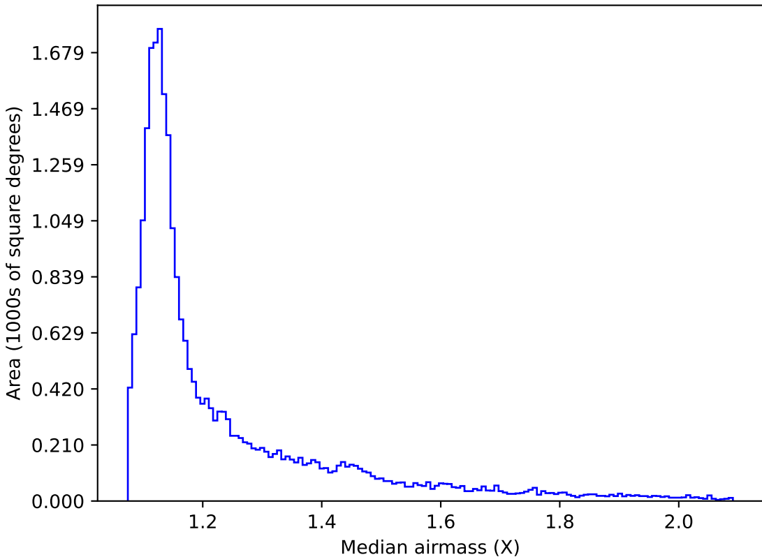
too_elab_r16_d2_griz_v3.4_10yrs Yr 1 all bands: Median airmass
