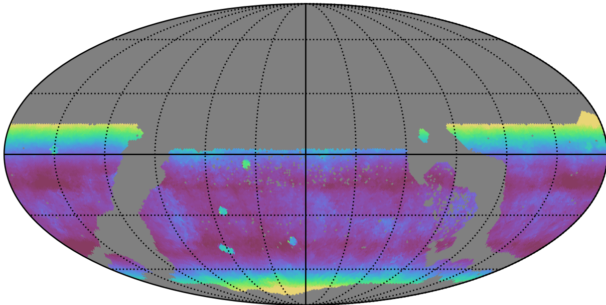
too_elab_r16_d2_griz_v3.4_10yrs WFD z band: Median airmass
