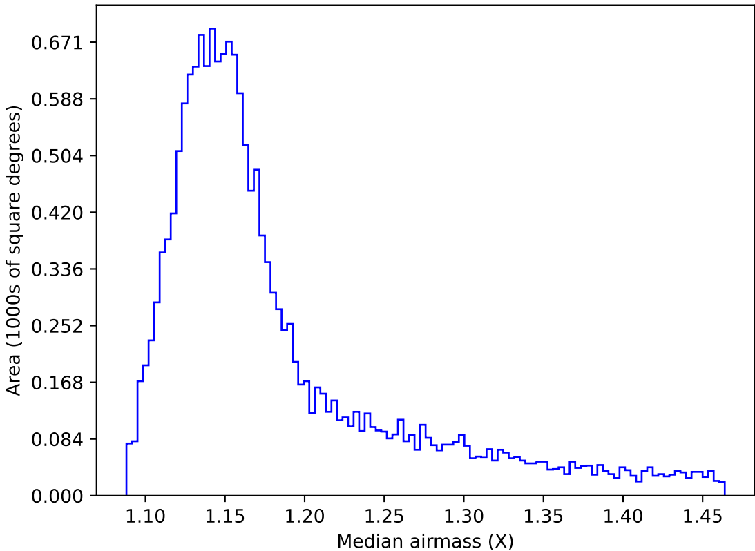
too_elab_r16_d2_griz_v3.4_10yrs WFD z band: Median airmass
