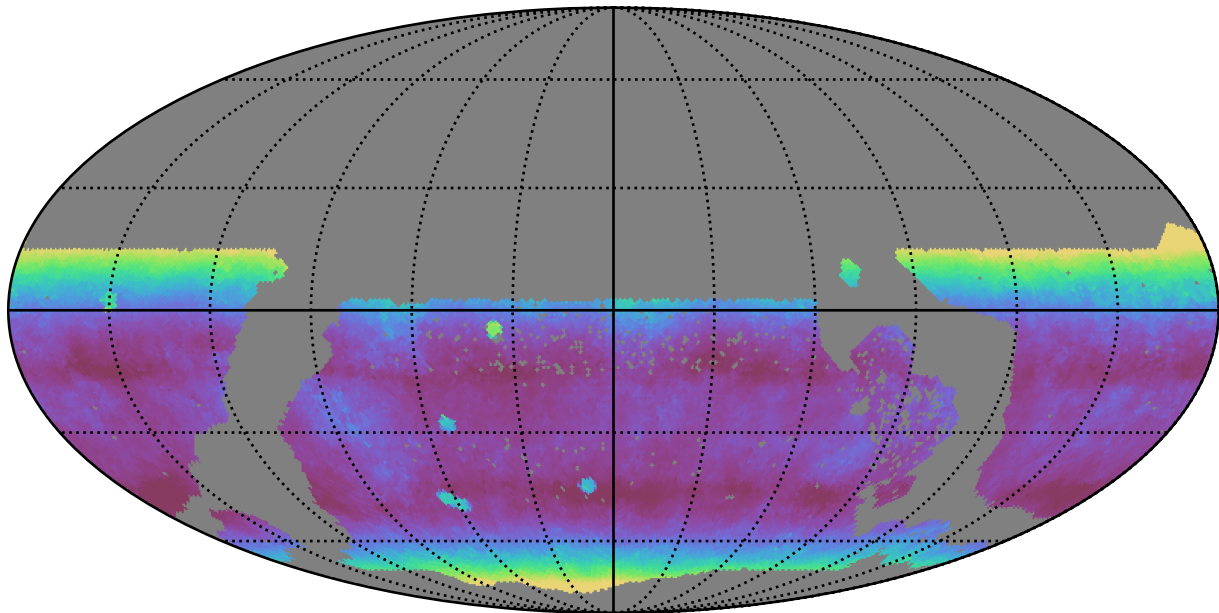
too_elab_r16_d2_griz_v3.4_10yrs WFD y band: Median airmass
