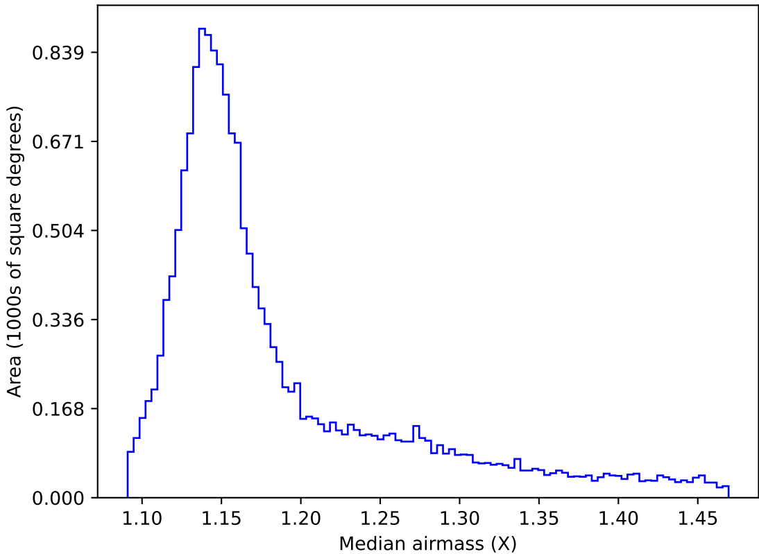
too_elab_r16_d2_griz_v3.4_10yrs WFD y band: Median airmass
