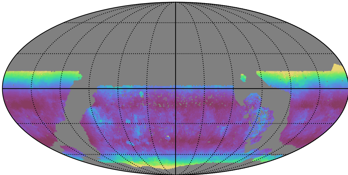
too_elab_r16_d2_griz_v3.4_10yrs WFD u band: Median airmass
