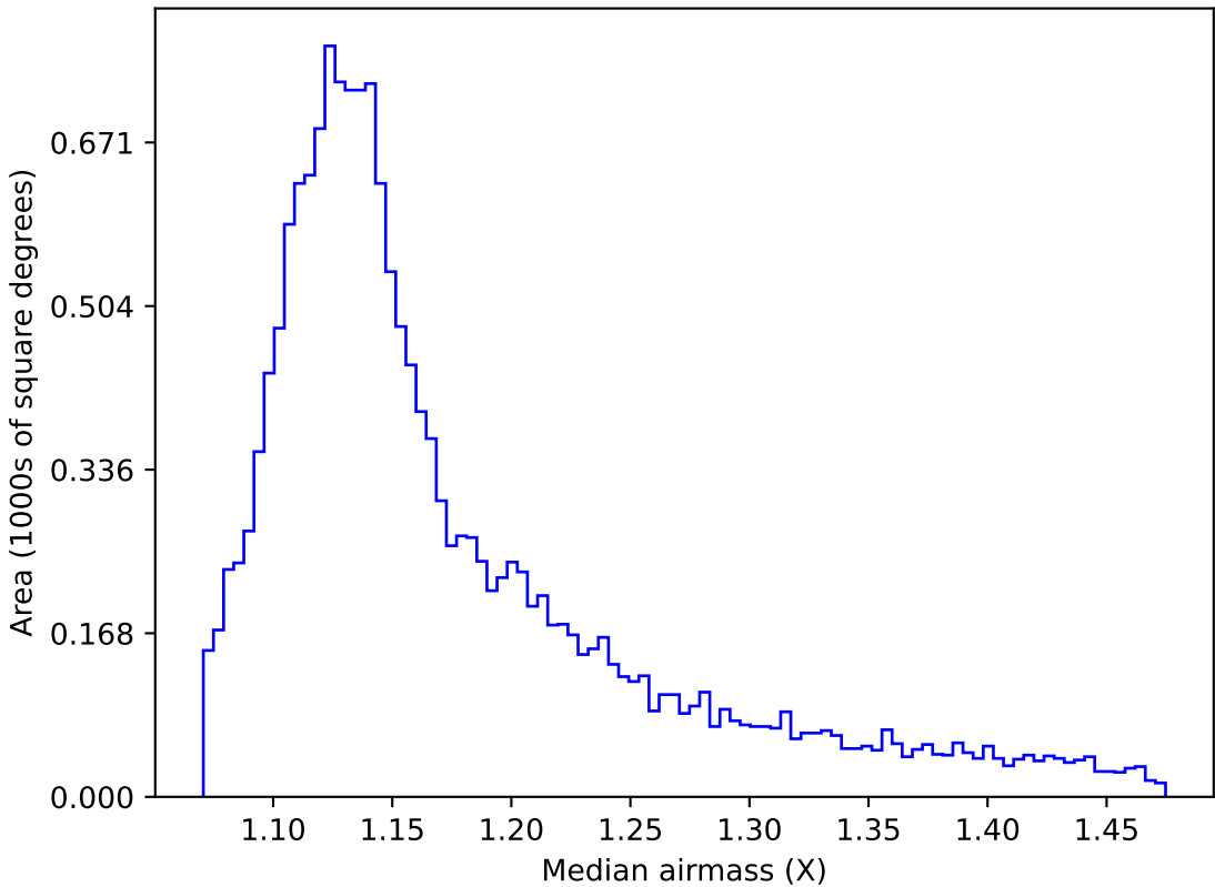
too_elab_r16_d2_griz_v3.4_10yrs WFD u band: Median airmass
