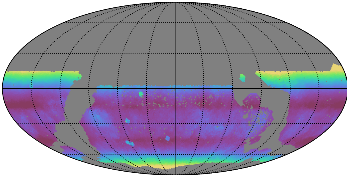
too_elab_r16_d2_griz_v3.4_10yrs WFD r band: Median airmass
