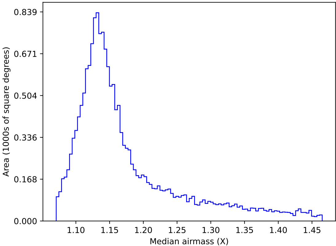
too_elab_r16_d2_griz_v3.4_10yrs WFD r band: Median airmass
