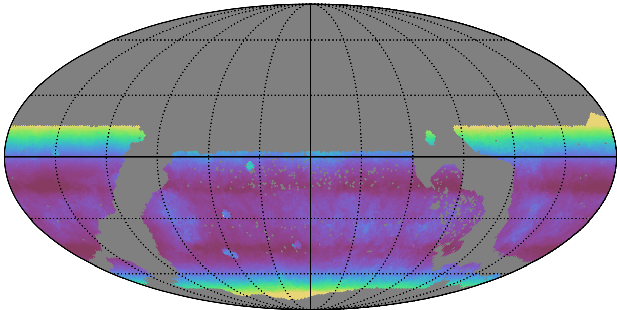
too_elab_r16_d2_griz_v3.4_10yrs WFD i band: Median airmass
