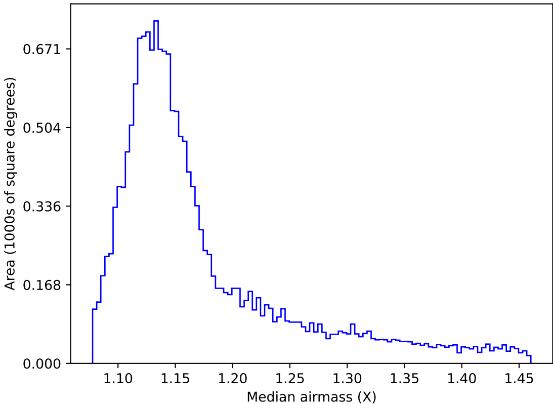
too_elab_r16_d2_griz_v3.4_10yrs WFD i band: Median airmass
