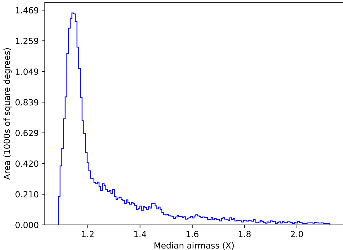
too_elab_r16_d2_griz_v3.4_10yrs All sky z band: Median airmass
