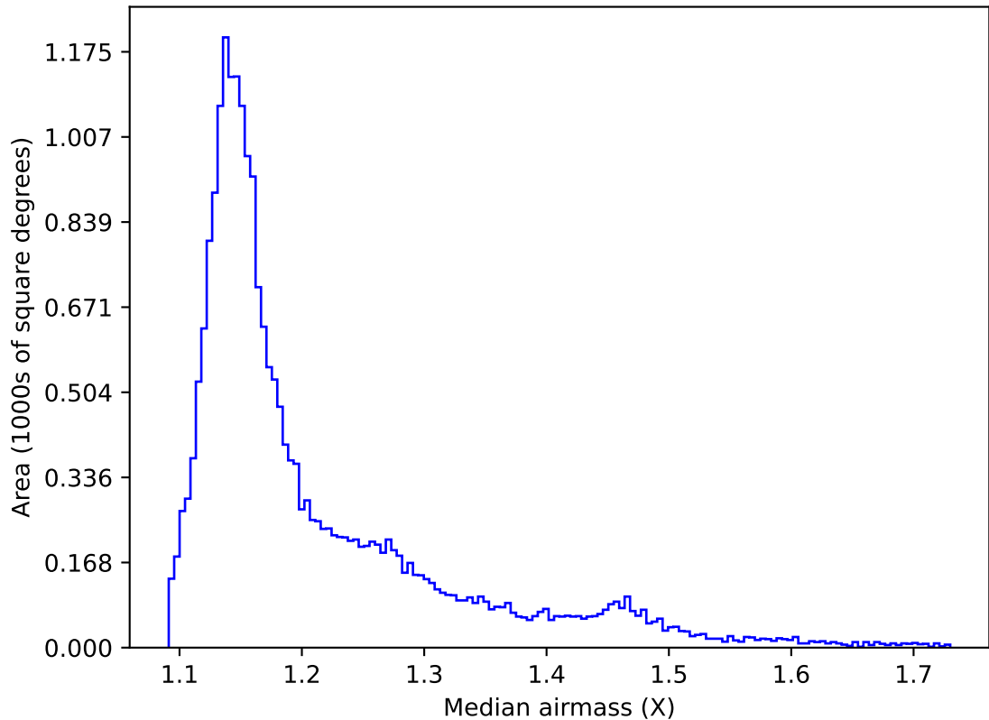
too_elab_r16_d2_griz_v3.4_10yrs All sky y band: Median airmass
