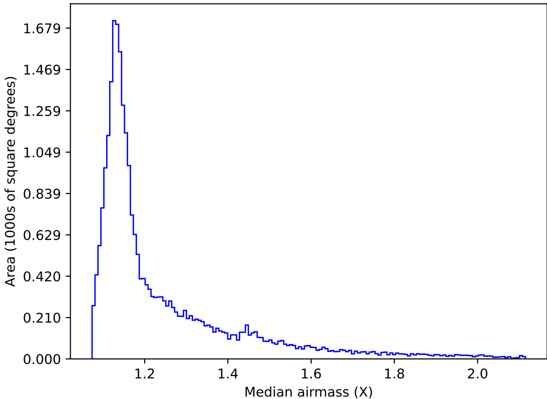
too_elab_r16_d2_griz_v3.4_10yrs All sky r band: Median airmass
