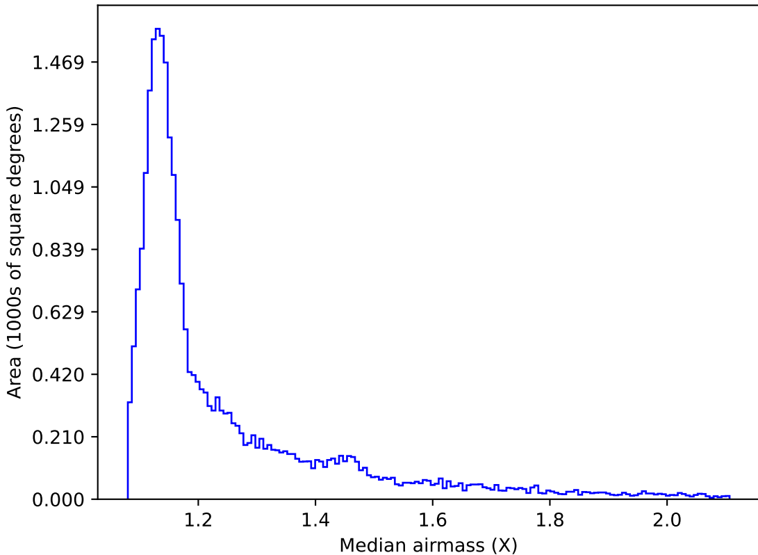
too_elab_r16_d2_griz_v3.4_10yrs All sky i band: Median airmass
