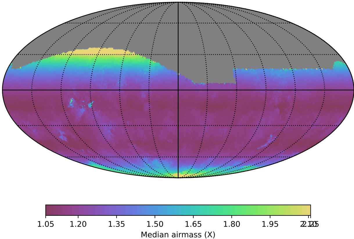
too_elab_r16_d2_griz_v3.4_10yrs All sky g band: Median airmass
