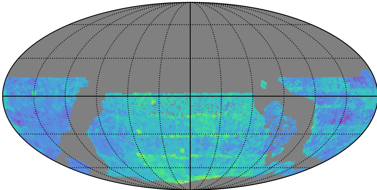
too_elab_r16_d2_griz_v3.4_10yrs WFD y band: Median Season Length
