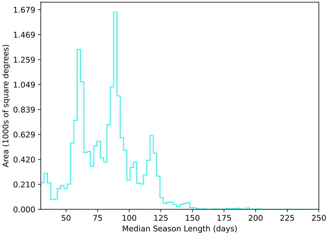
too_elab_r16_d2_griz_v3.4_10yrs WFD u band: Median Season Length
