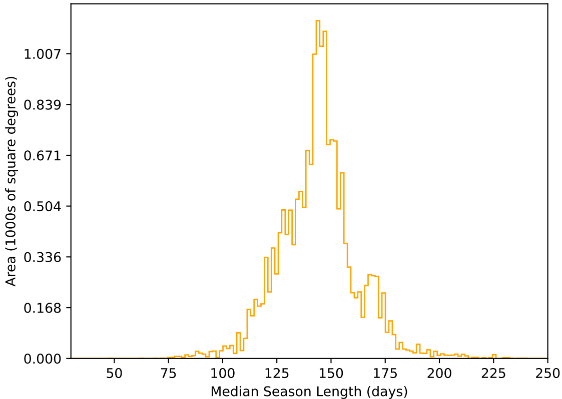
too_elab_r16_d2_griz_v3.4_10yrs WFD r band: Median Season Length
