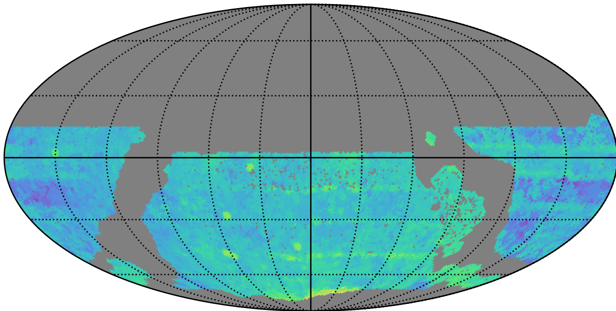
too_elab_r16_d2_griz_v3.4_10yrs WFD i band: Median Season Length
