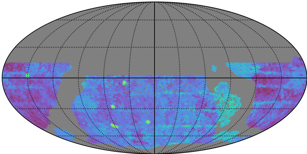
too_elab_r16_d2_griz_v3.4_10yrs WFD g band: Median Season Length
