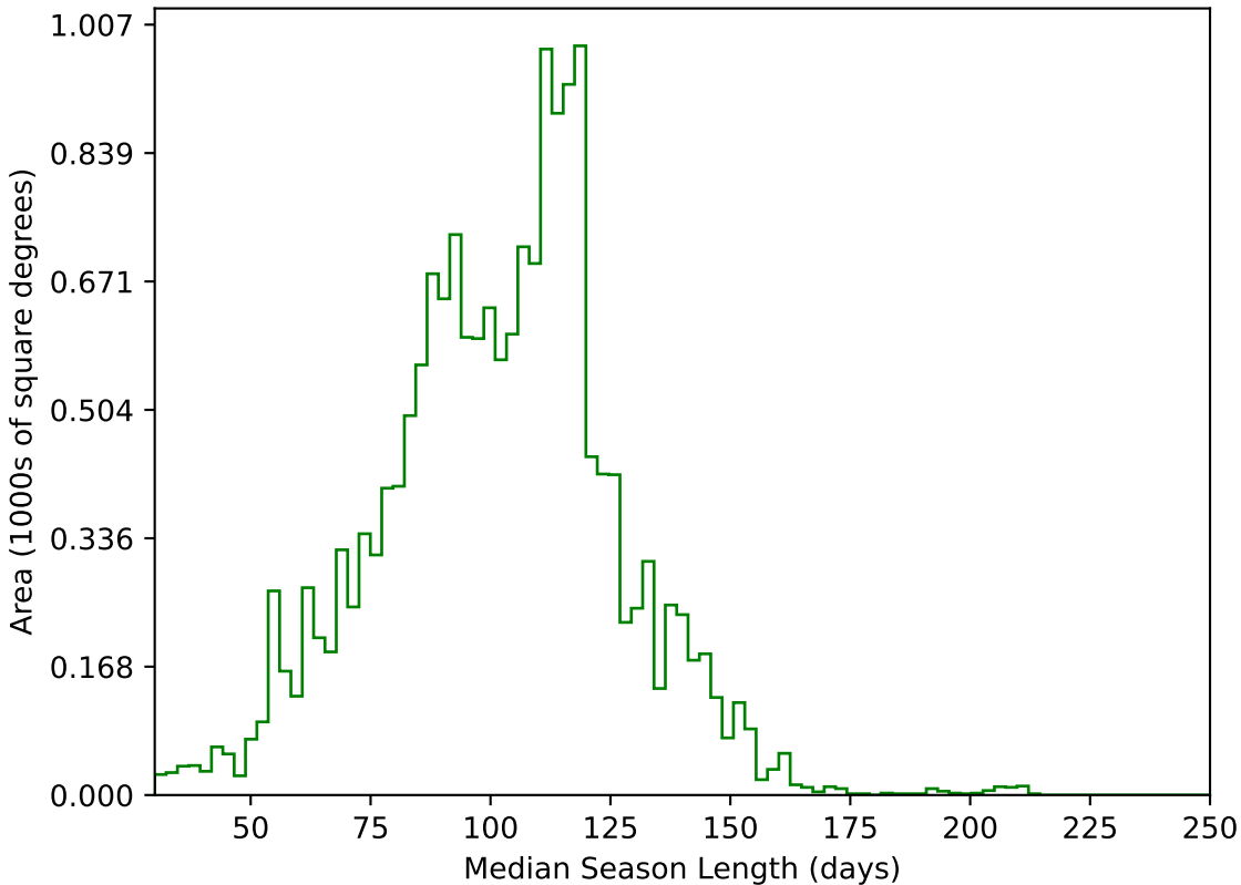
too_elab_r16_d2_griz_v3.4_10yrs WFD g band: Median Season Length
