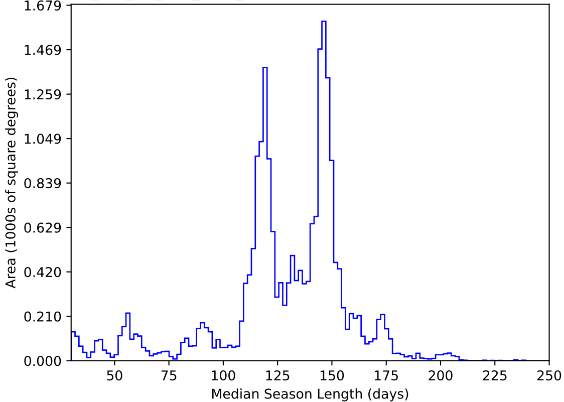
too_elab_r16_d2_griz_v3.4_10yrs All sky y band: Median Season Length
