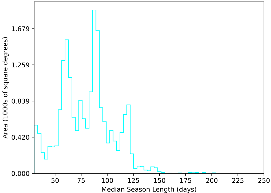
too_elab_r16_d2_griz_v3.4_10yrs All sky u band: Median Season Length
