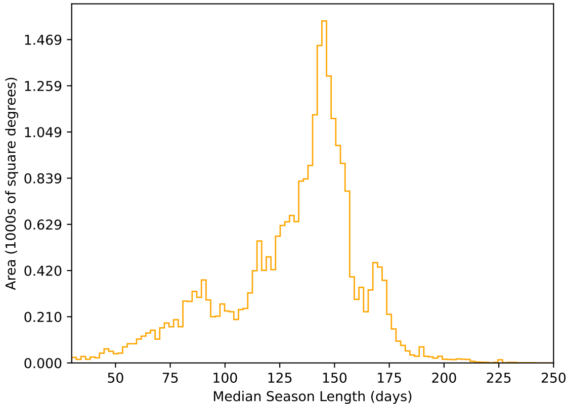
too_elab_r16_d2_griz_v3.4_10yrs All sky r band: Median Season Length
