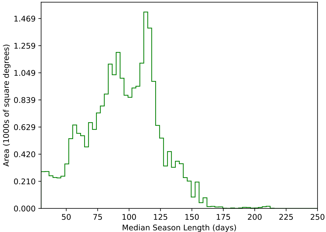
too_elab_r16_d2_griz_v3.4_10yrs All sky g band: Median Season Length
