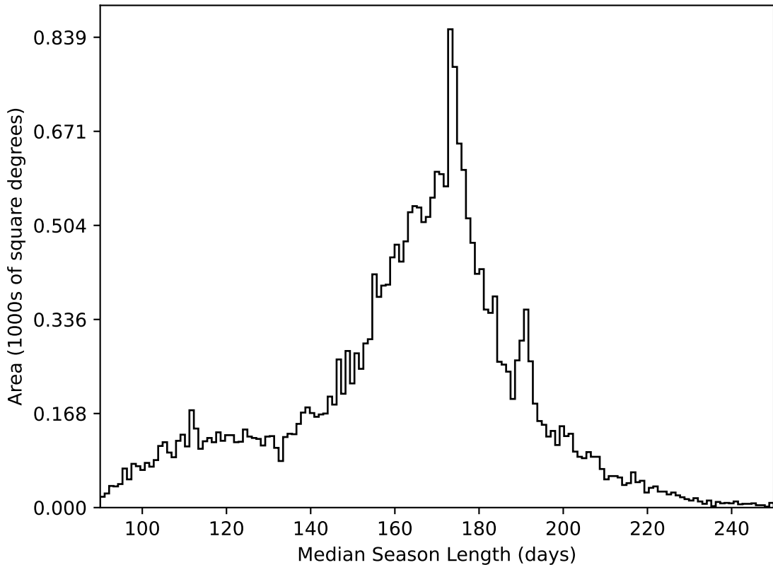
too_elab_r16_d2_griz_v3.4_10yrs All sky all bands: Median Season Length
