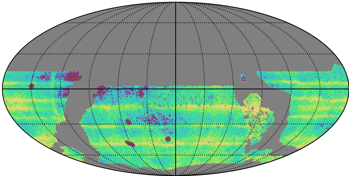
too_elab_r16_d2_griz_v3.4_10yrs WFD: Median Intra-Night Gap
