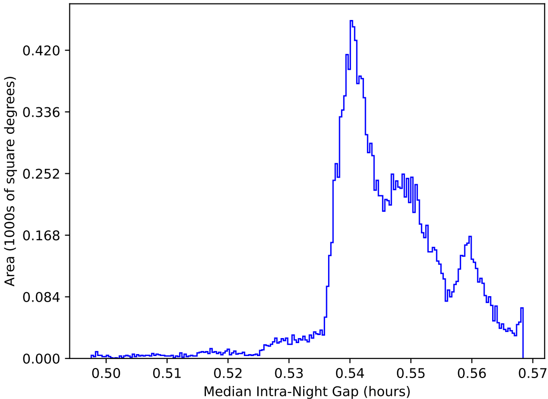
too_elab_r16_d2_griz_v3.4_10yrs WFD: Median Intra-Night Gap
