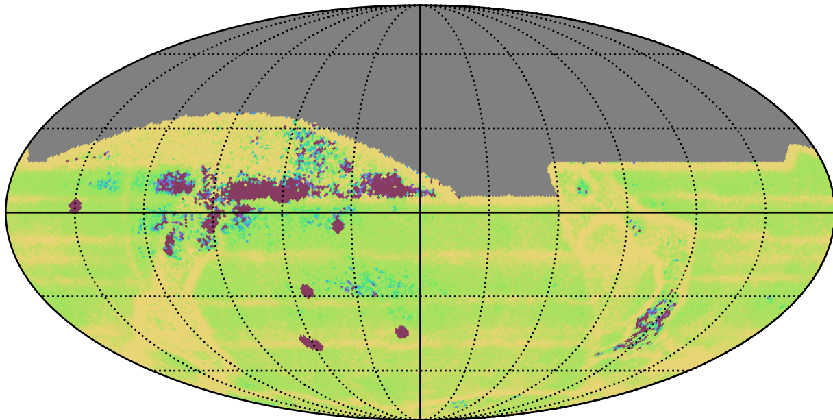
too_elab_r16_d2_griz_v3.4_10yrs All sky: Median Intra-Night Gap
