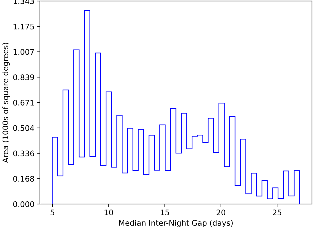
too_elab_r16_d2_griz_v3.4_10yrs WFD y band: Median Inter-Night Gap
