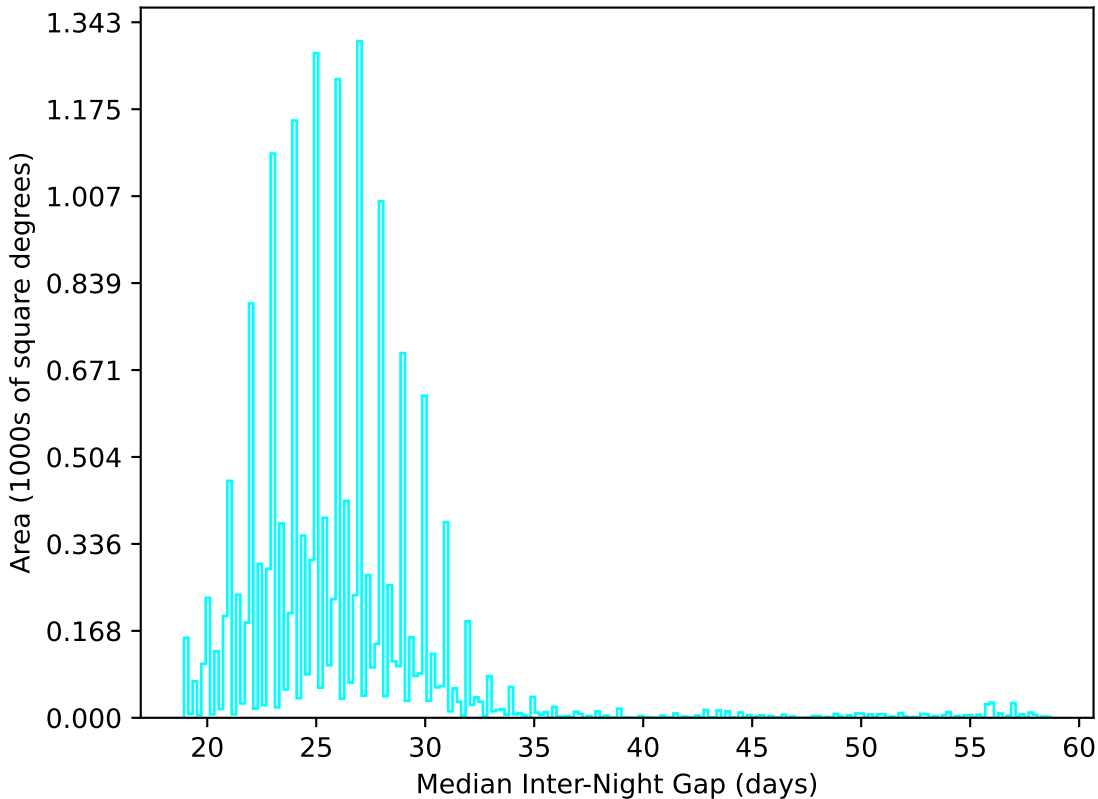
too_elab_r16_d2_griz_v3.4_10yrs WFD u band: Median Inter-Night Gap
