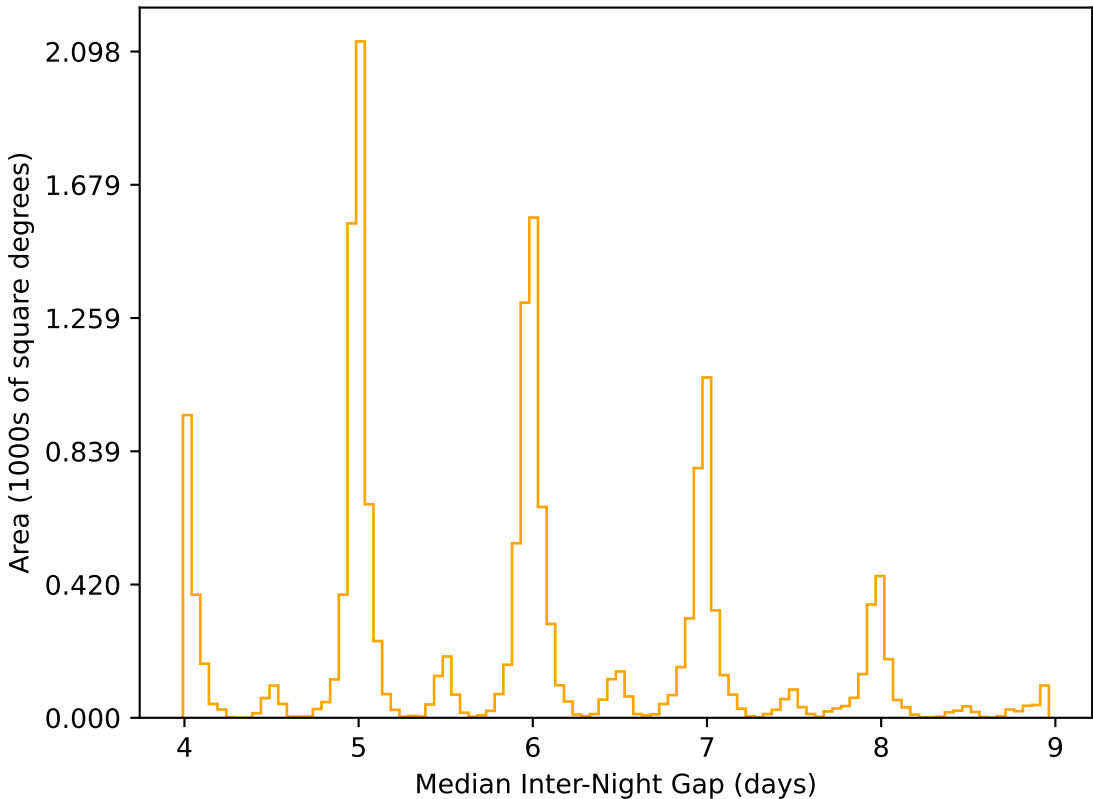
too_elab_r16_d2_griz_v3.4_10yrs WFD r band: Median Inter-Night Gap
