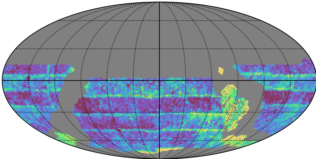
too_elab_r16_d2_griz_v3.4_10yrs WFD i band: Median Inter-Night Gap
