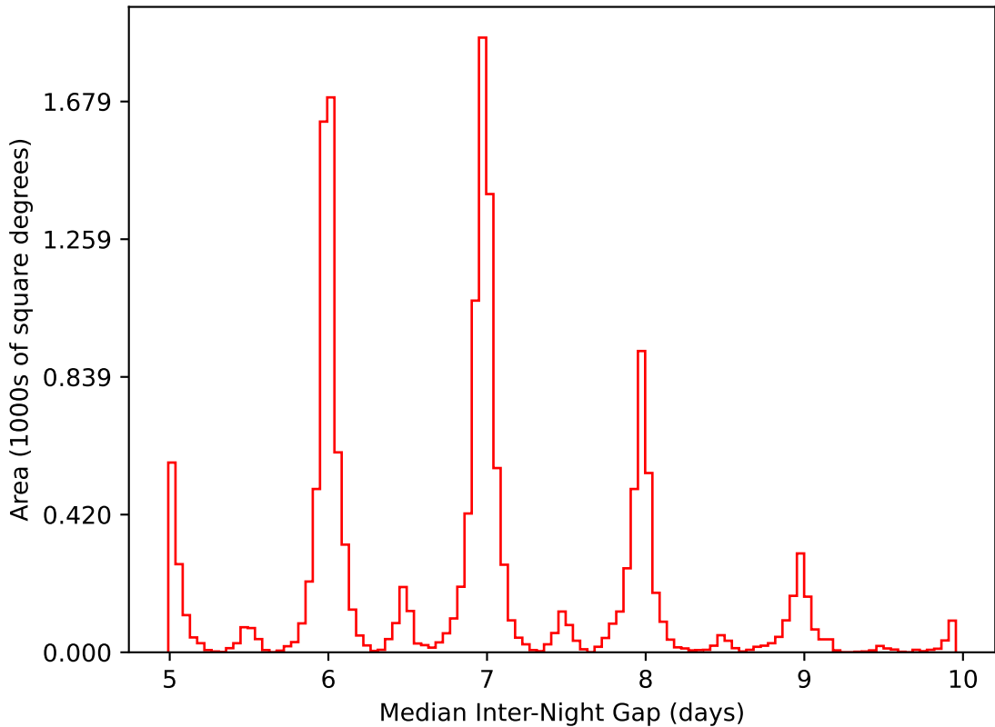
too_elab_r16_d2_griz_v3.4_10yrs WFD i band: Median Inter-Night Gap
