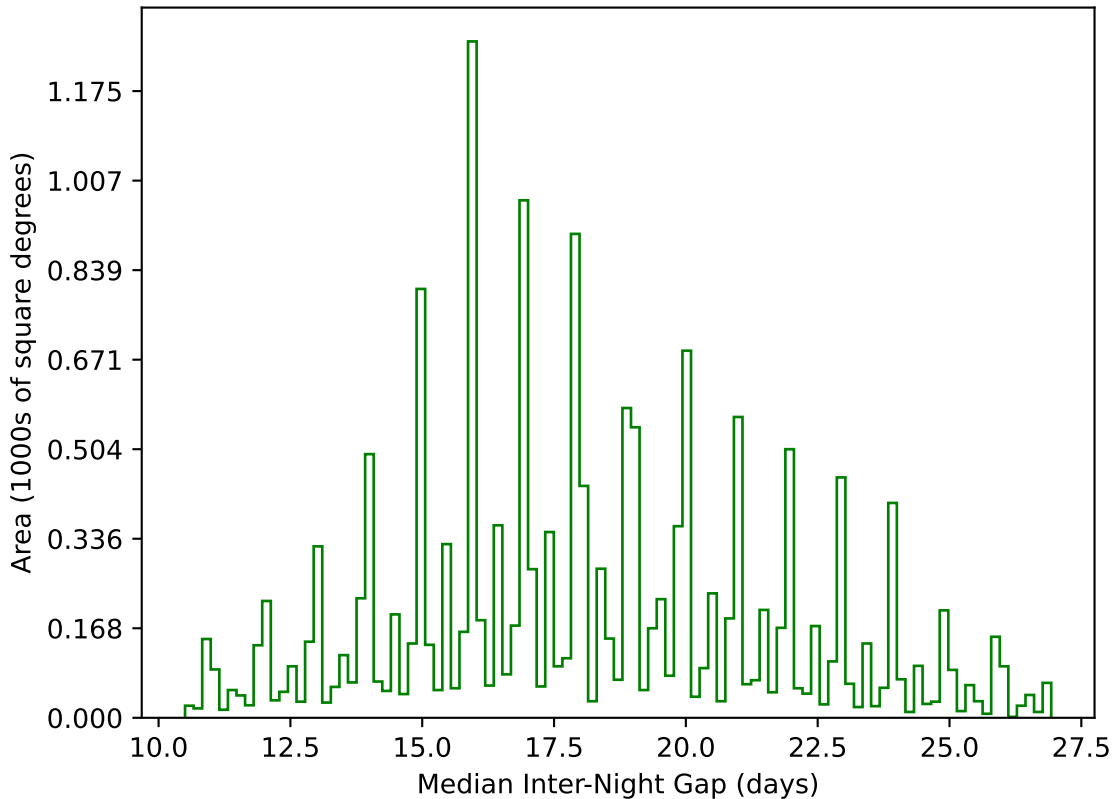
too_elab_r16_d2_griz_v3.4_10yrs WFD g band: Median Inter-Night Gap
