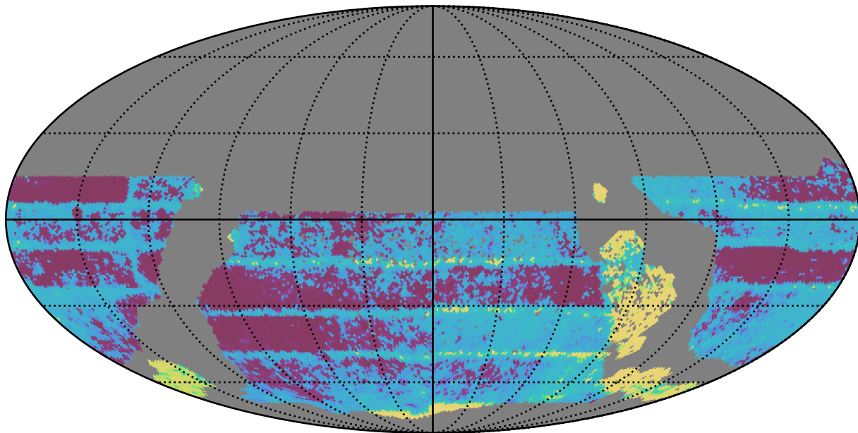
too_elab_r16_d2_griz_v3.4_10yrs WFD all bands: Median Inter-Night Gap
