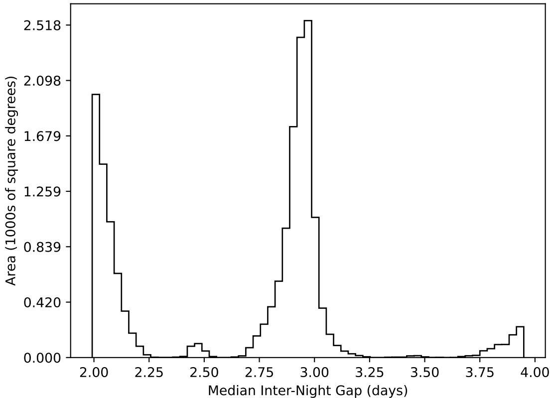
too_elab_r16_d2_griz_v3.4_10yrs WFD all bands: Median Inter-Night Gap
