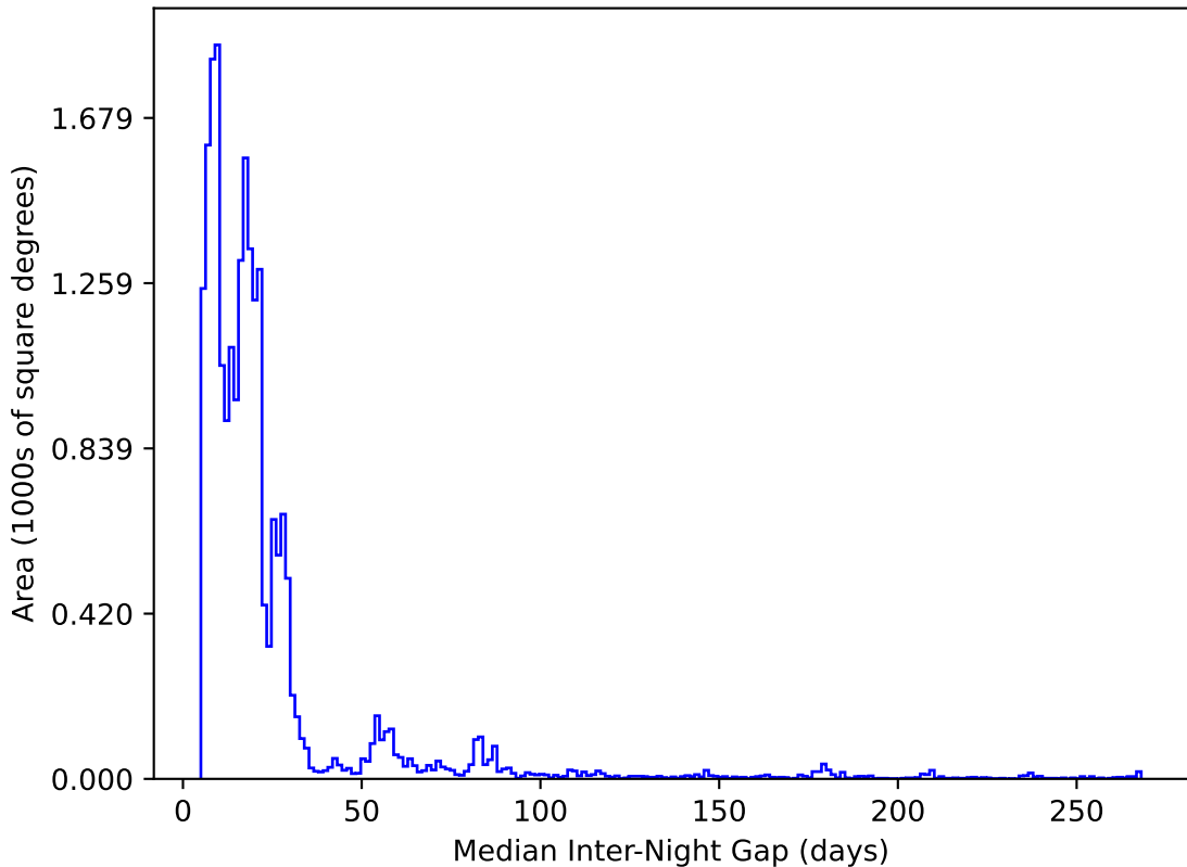
too_elab_r16_d2_griz_v3.4_10yrs All sky y band: Median Inter-Night Gap
