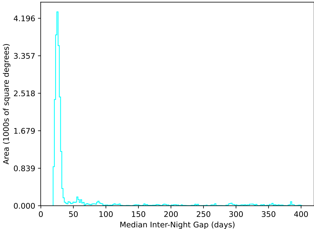
too_elab_r16_d2_griz_v3.4_10yrs All sky u band: Median Inter-Night Gap
