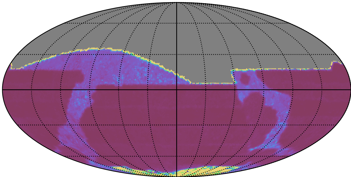
too_elab_r16_d2_griz_v3.4_10yrs All sky r band: Median Inter-Night Gap
