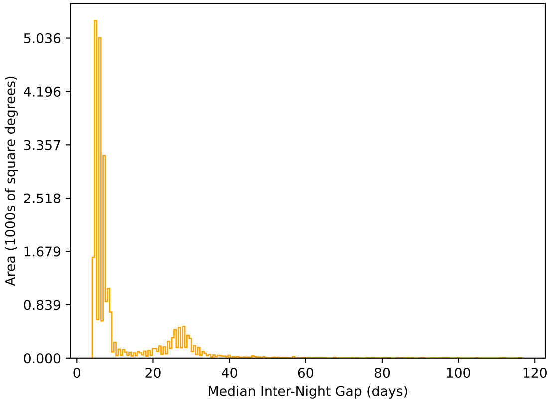
too_elab_r16_d2_griz_v3.4_10yrs All sky r band: Median Inter-Night Gap
