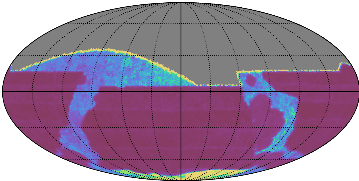
too_elab_r16_d2_griz_v3.4_10yrs All sky i band: Median Inter-Night Gap
