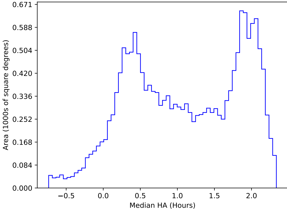
too_elab_r16_d2_griz_v3.4_10yrs WFD z band: Median HA
